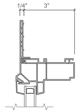
3-1/4-in. double-wall flush-flange
