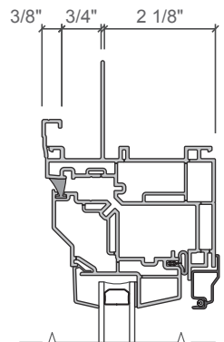
3-1/4-in. nail fin with j-channel frame
