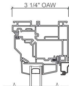
3-1/4-in. block frame
