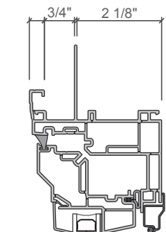
3-1/4-in. nail fin with j-channel frame
