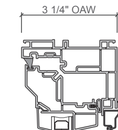
3-1/4-in. block frame
