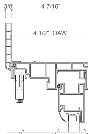
4-1/2-in. flush-flange frame
