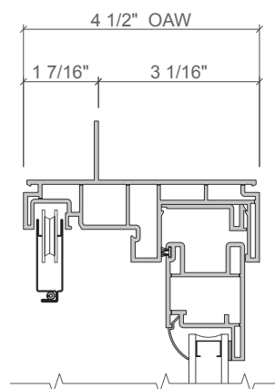
4-1/2-in. nail fin frame
